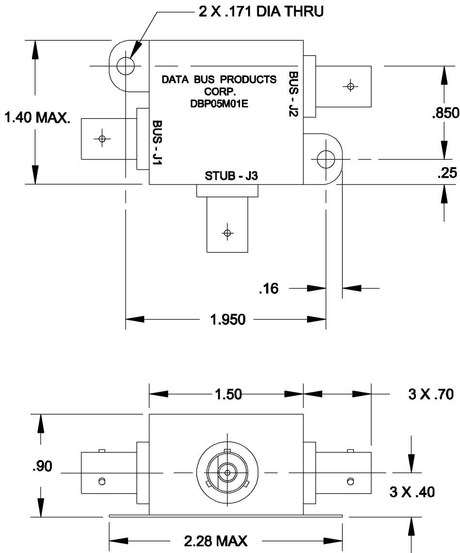
INTERFACE CONTROL DRAWING
